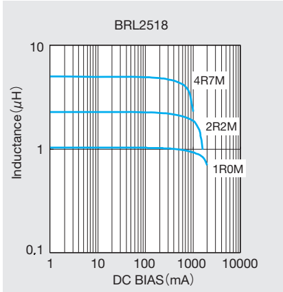
直流重量特性例 DC Bias characteristics (Measured by HP4285A)
