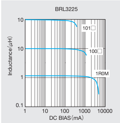
直流重量特性例 DC Bias characteristics (Measured by HP4285A)
